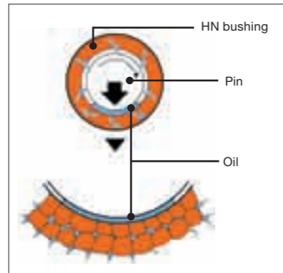
Job-Proven HN Bushings The field-proven HN bushing, a Hitachi original, is utilized at each front pin joint to reduce jerking and servicing. Lubricating interval is a long 500 hours
