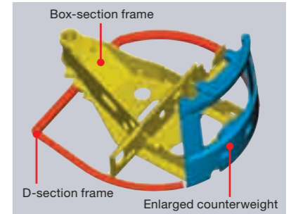
Enlarged Counterweight and Weighted Undercarriage The newly developed box-section frame is adopted, combining low weight and high durability. The enlarged counterweight and weighted undercarriage help lower the center of gravity and increase stability.
