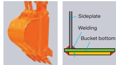
Durable Flat-Bottom Bucket The flat-bottom bucket is provided standard to minimize bucket bottom wear. Wide wear plates are welded to the bucket bottom for increased durability.
